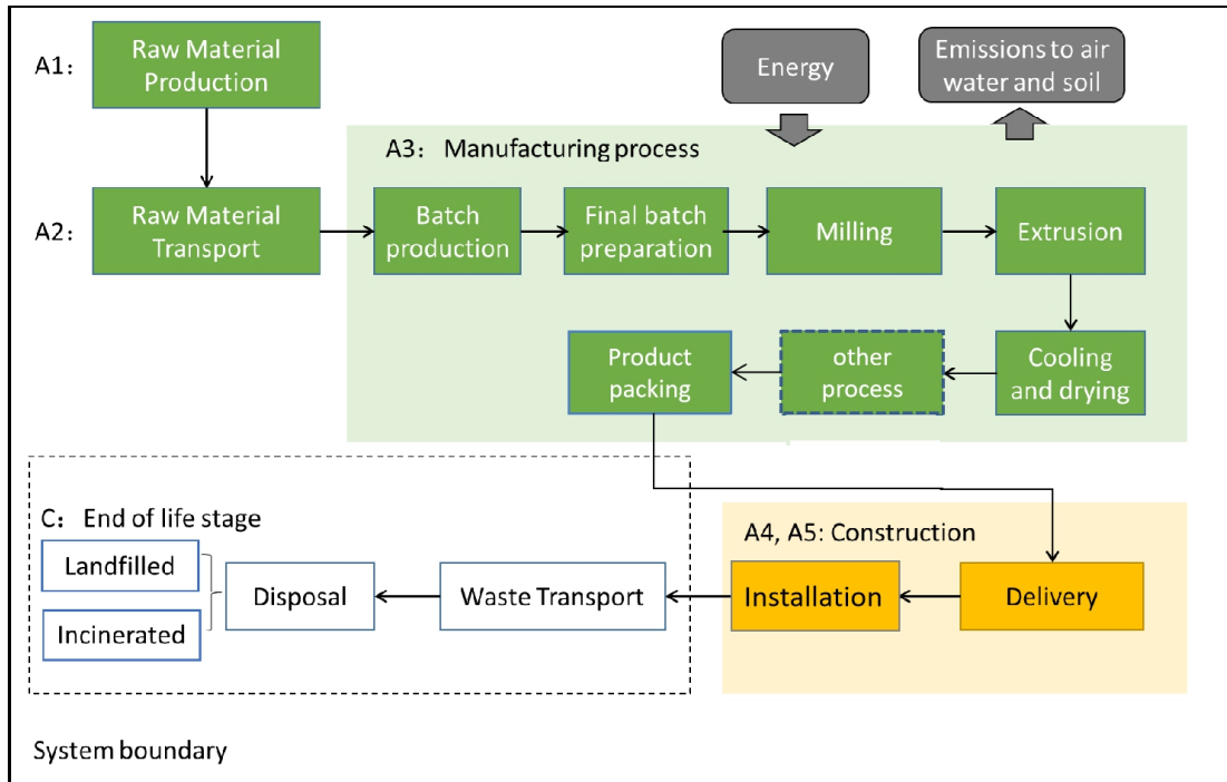
Figure 3: System boundary of insulation products
