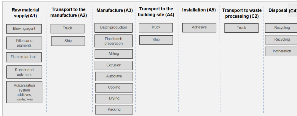
Figure 2: The flow diagram of K-FLEX non-pipe insulation products
